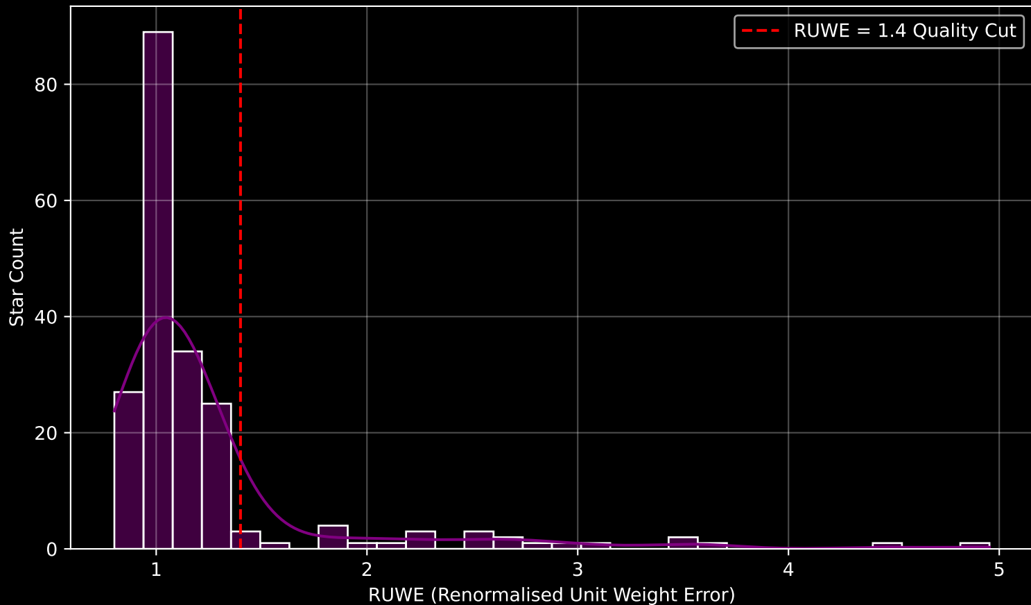
GAPOGEE DR17 Field [058-39_MGA] RUWE Distribution (n= 201)
