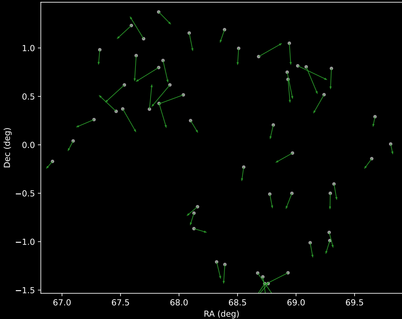
APOGEE DR17 Cluster 4 Proper Motion Vectors (n=52)
