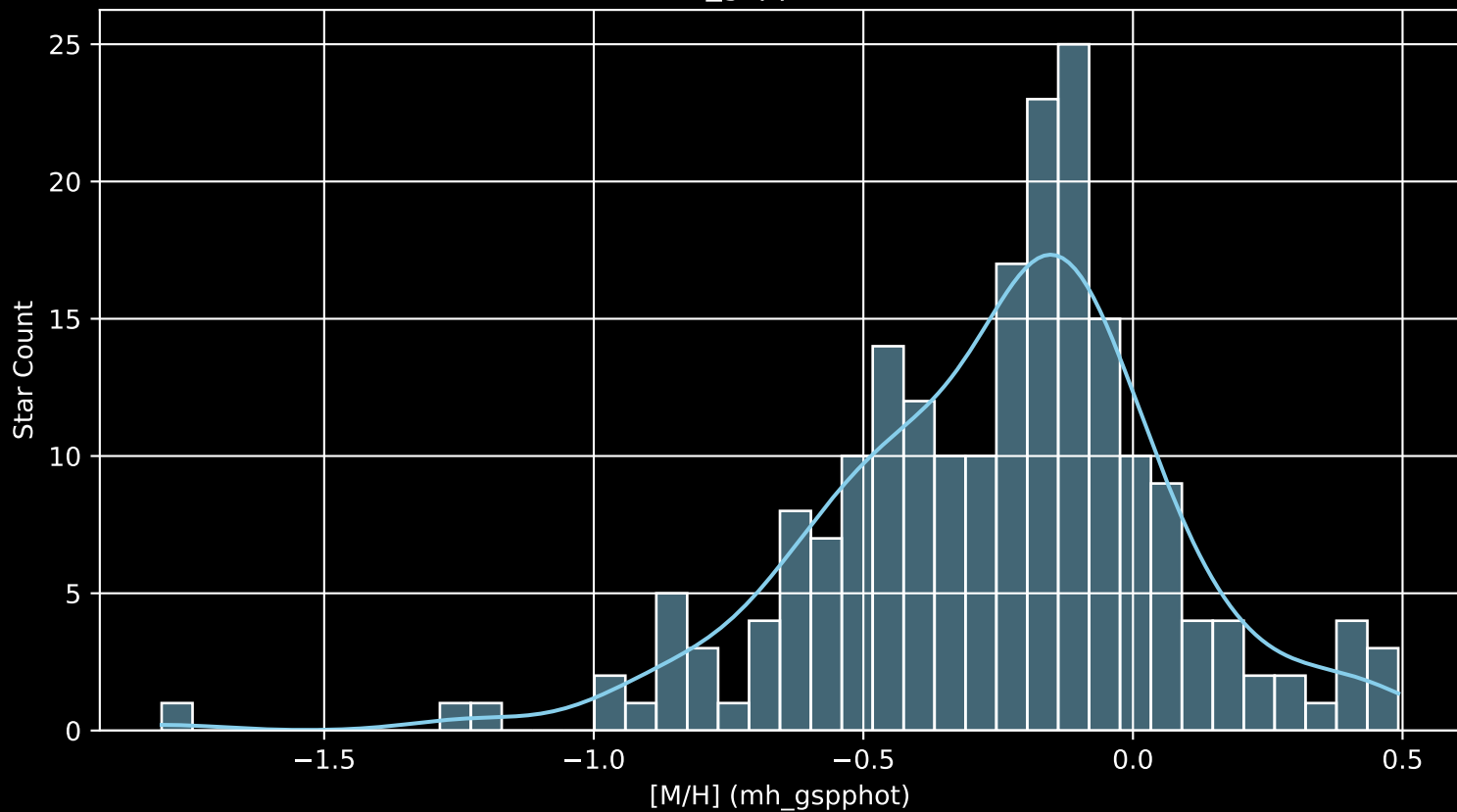
APOGEE DR17 Field: [058-39_MGA [M/H] (mh_gspphot) (n= 209)
