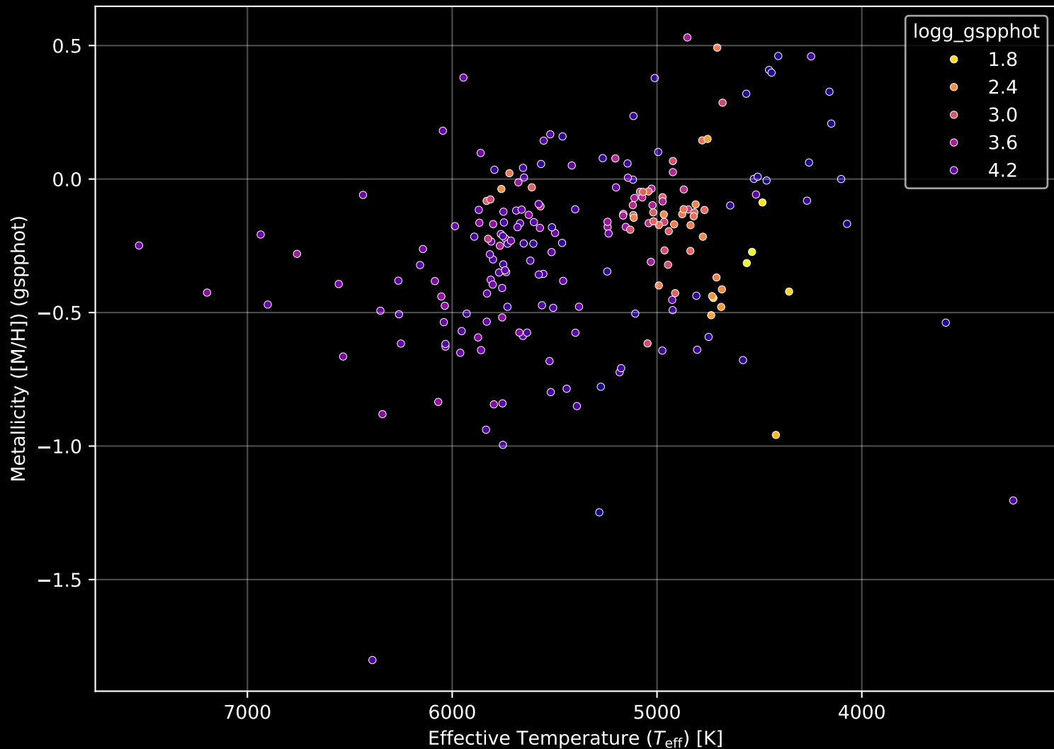
APOGEE DR17 Field: [058-39_MGA] Stellar Population Parameters (n= 210)
