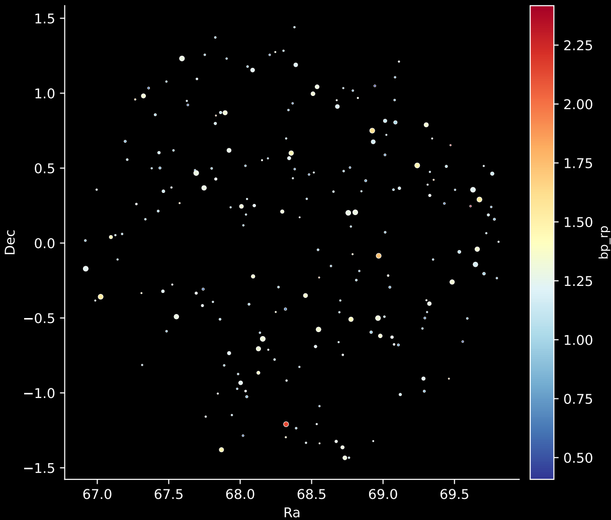
APOGEE DR17 Field: [058-39_MGA] Stars: 210
