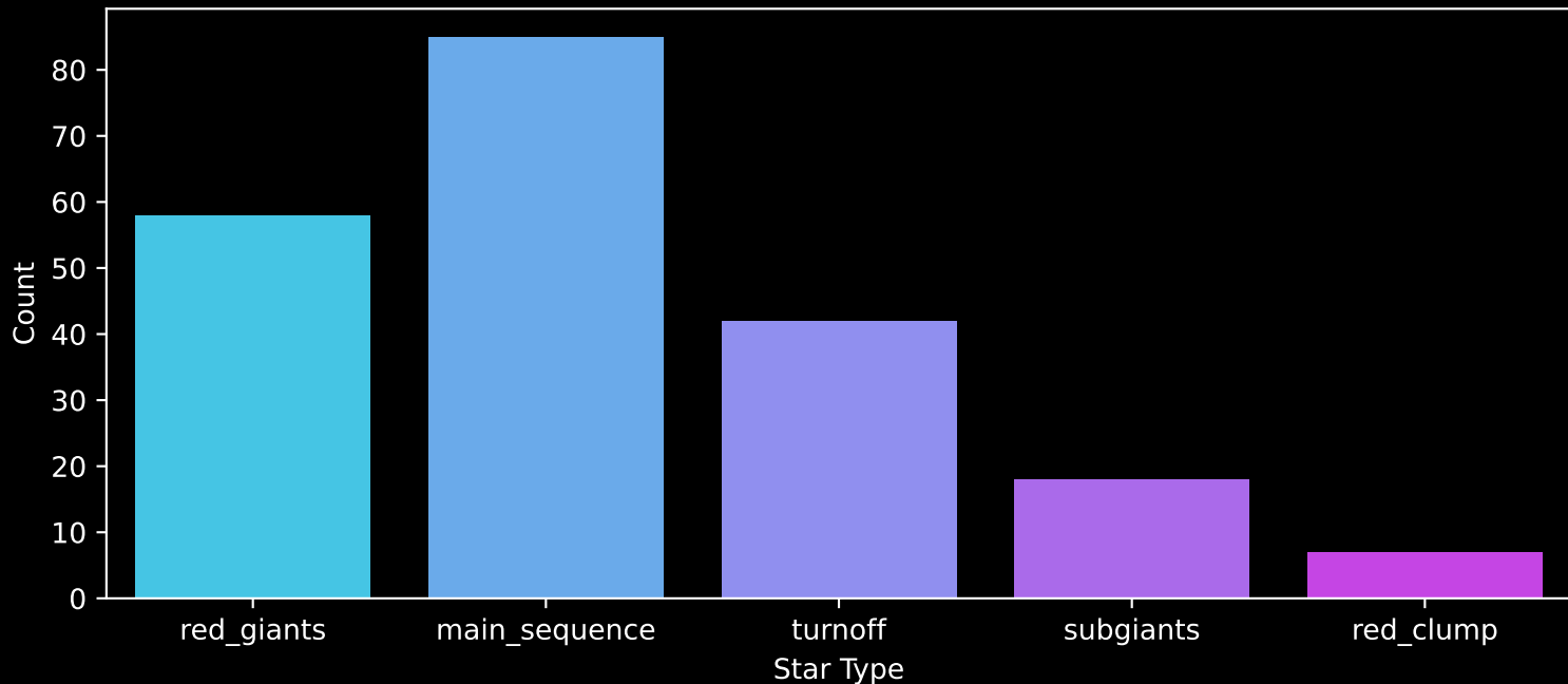
APOGEE DR17 Field: [058-39_MGA] Count plot of Star Type
