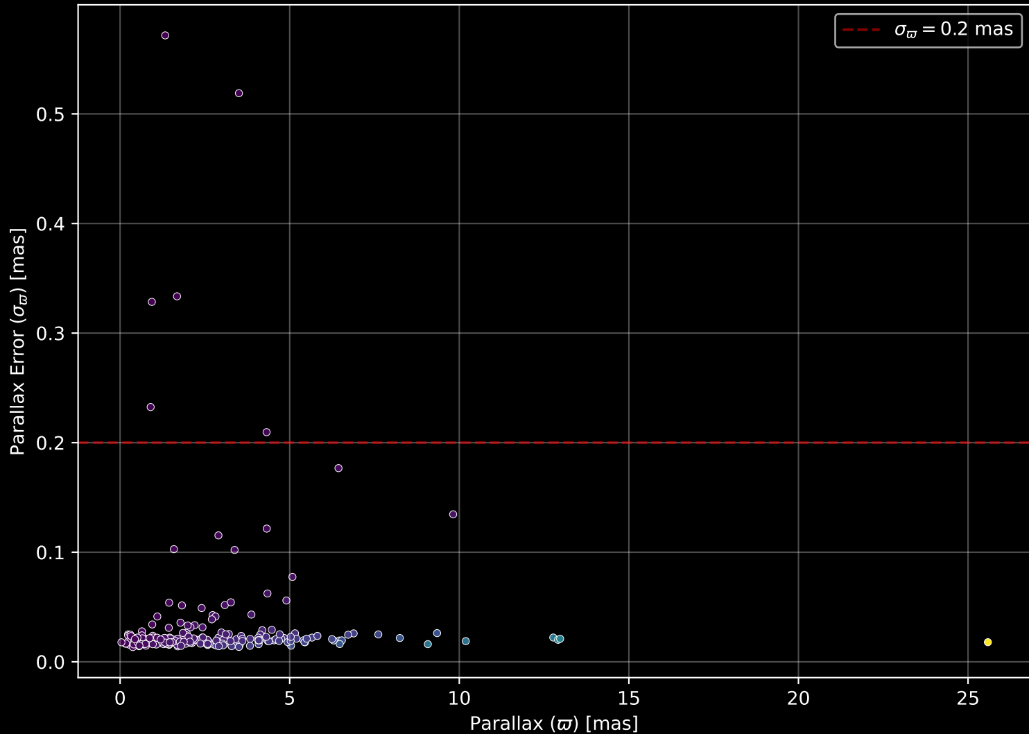
APOGEE DR17 Field: [058-39_MGA] Parallax Quality (n= 210)
