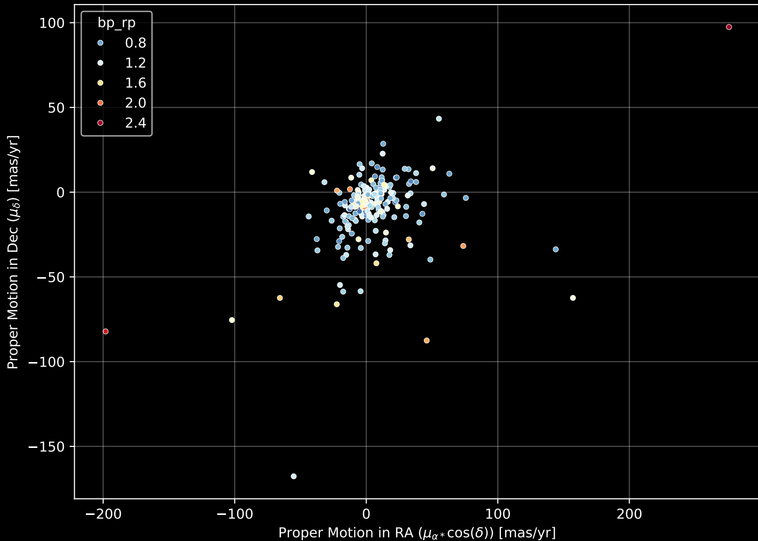
APOGEE DR17 Field: [058-39_MGA] Proper Motion Diagram (n= 210)
